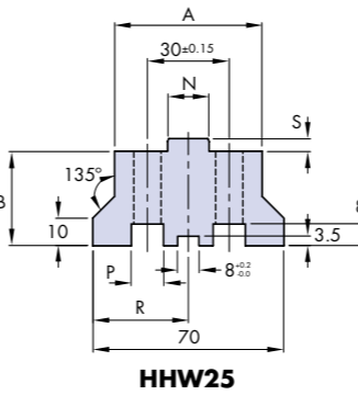
High Wide Back Plate
